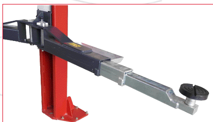
4 three-section symmetric arms.
