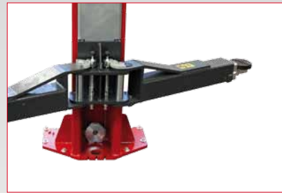
Toothed sector arm rotation stop system
